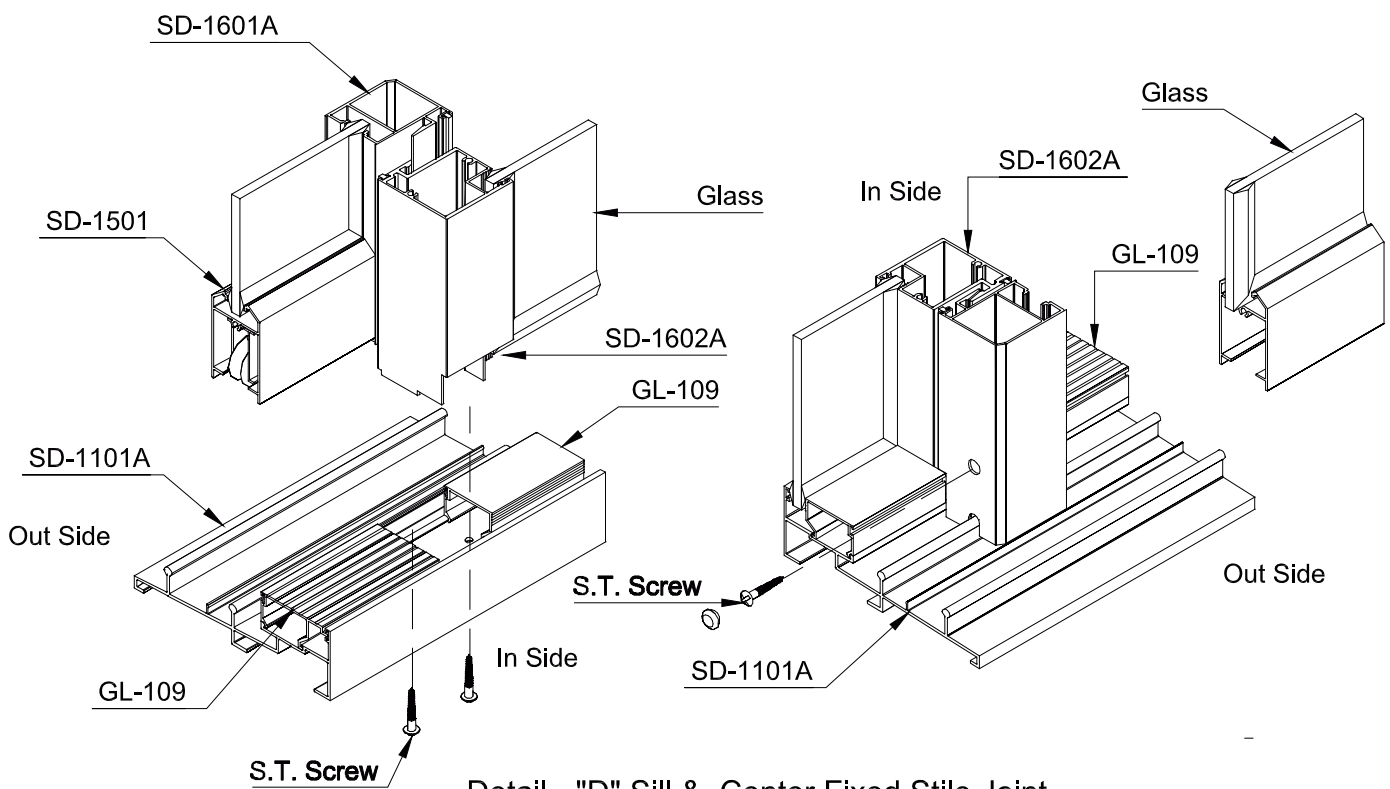
Detail - "D" Sill & Center Fixed Stile Joint
