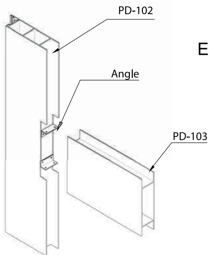
Assembly - Middle Bar
