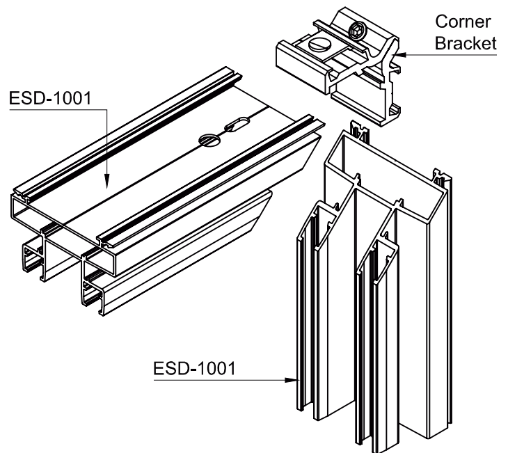
Detail- "A" Head & Jumb Corner Joint 45°
