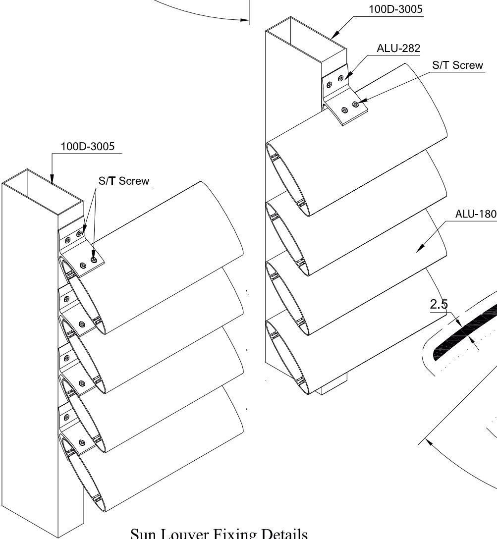
Sun Louver Fixing Details
