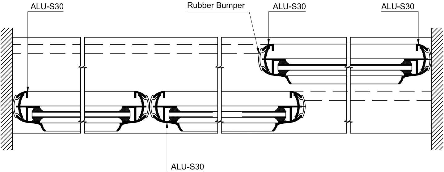
SECTION :- B-B
