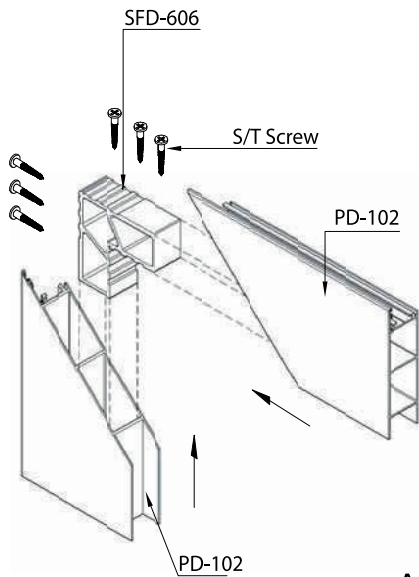
Detail - "B" Sash Corner 45° joint
