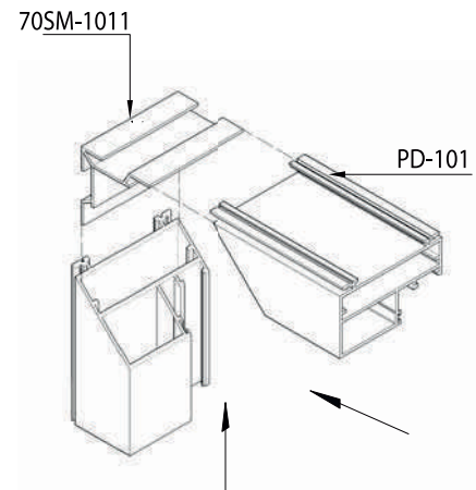
Detail - "A" Head & Jamb Corner Joint
