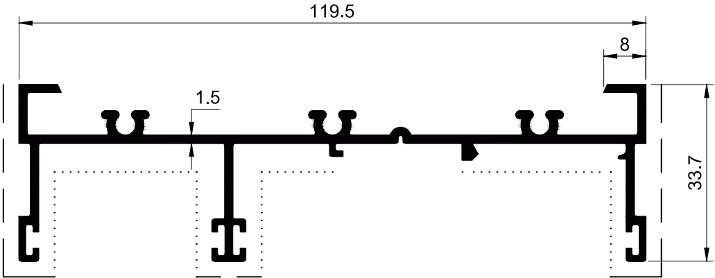
SECTION NO. - 80S-2001A EST. WEIGHT - 1.168 KG./M.
