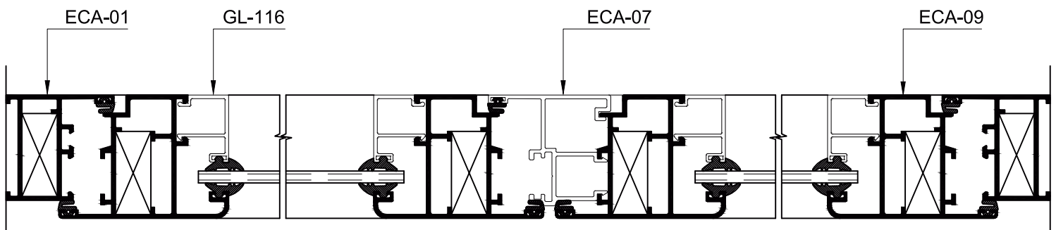
SECTION :- B-B
