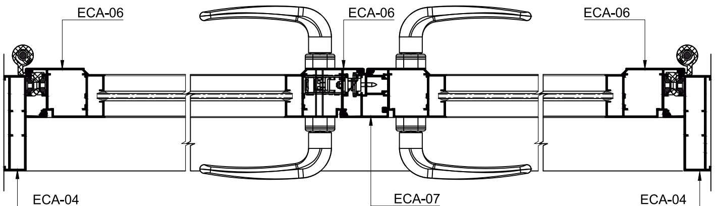
Section :- B-B
