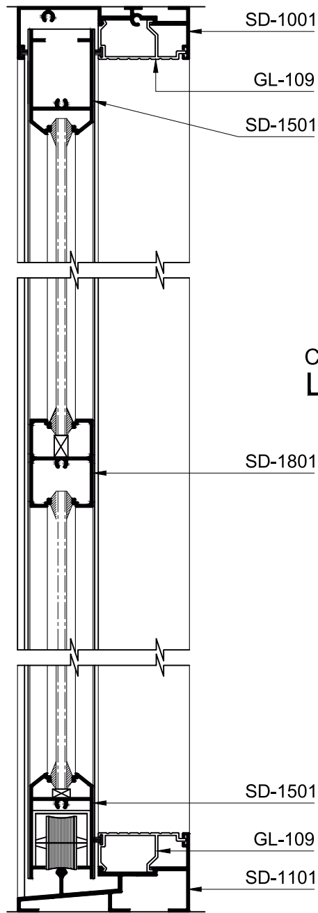
SECTION :- A - A
