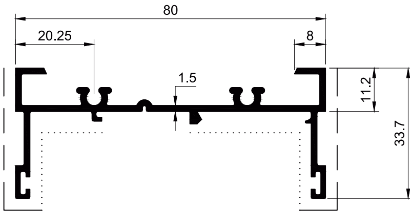
SECTION NO. - 80S-2001 EST. WEIGHT - 0.823 KG./M.
