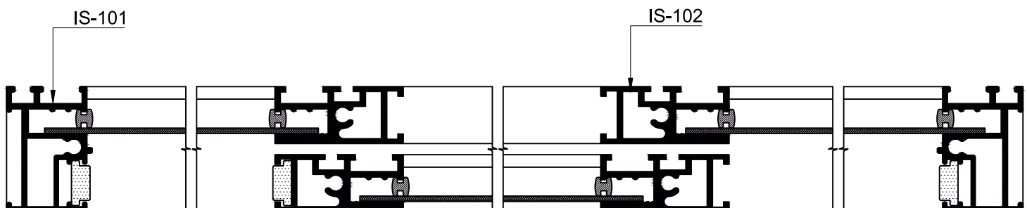
SECTION :- B-B
