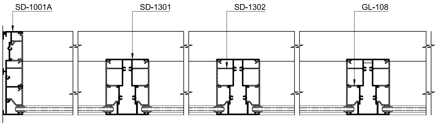
Section :- E-E
