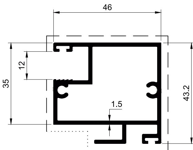
SECTION NO. - 80S-2602 EST. WEIGHT - 0.941 KG./M.
