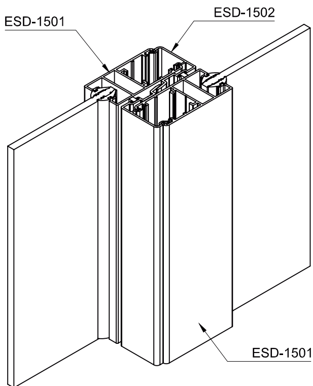
Detail- "C" Sash Inter Lock
